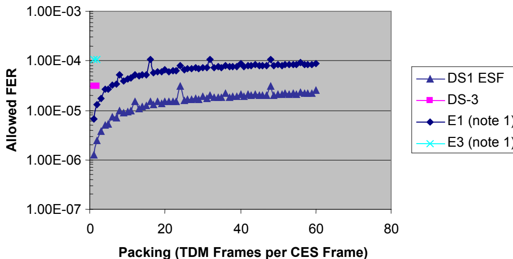
Figure 18: Relationship between Packing and FER for 0.01% SES
