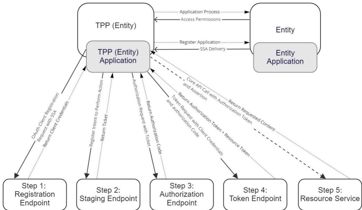
Figure 4 – MEF LSO APIs Security Architecture
